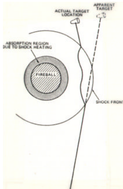
Refraction
